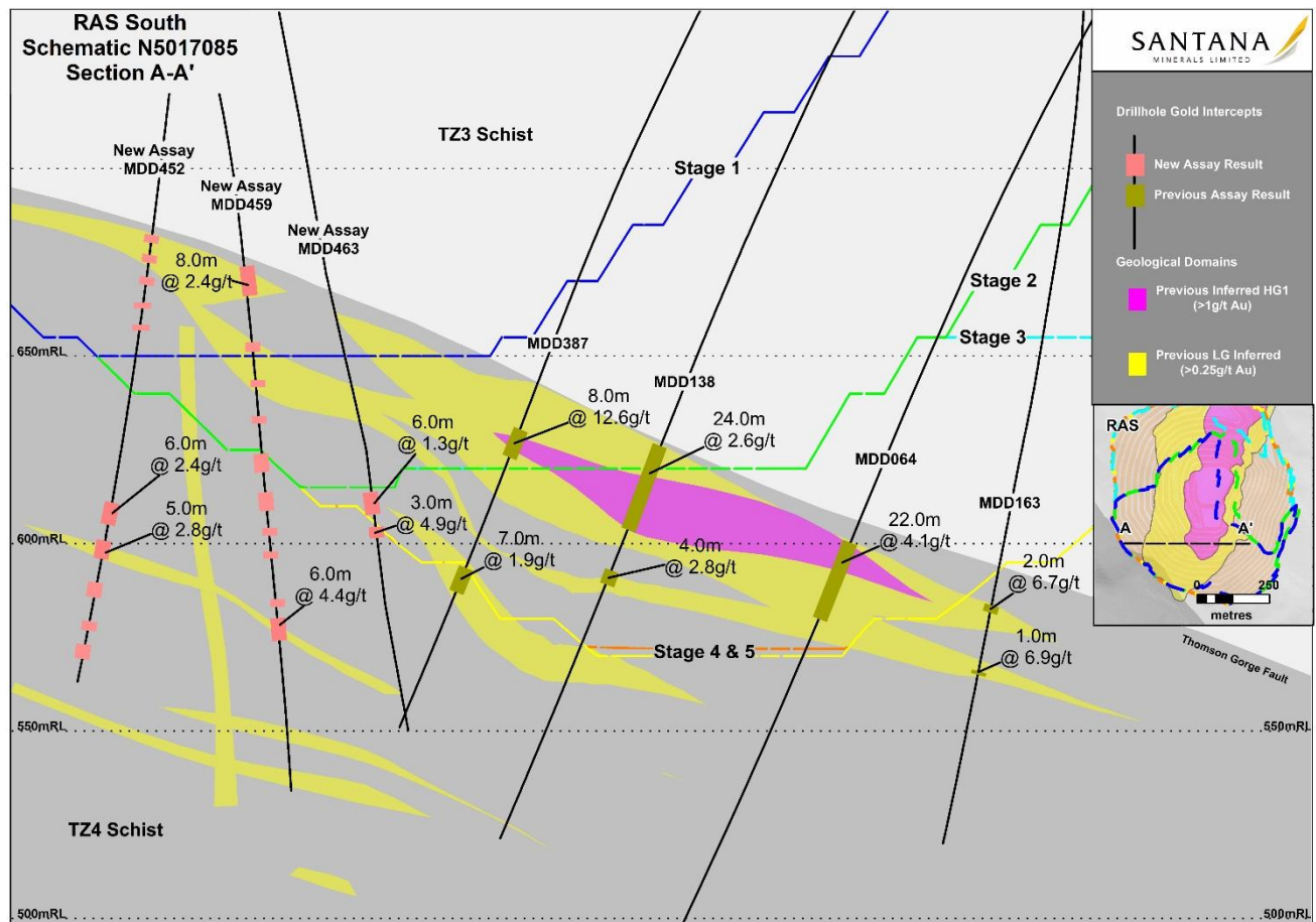
Figure 4. Schematic cross section at 5017085N showing new drilling and intercepts below pit design.
