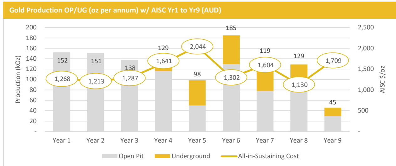
Figure 3. Production Profile OP/UG w/AISC estimates at A$4,000/oz.
